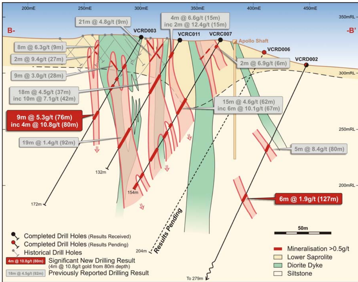
Figure 4 Apollo Drill Section. (See B-B' on Figure 2)
